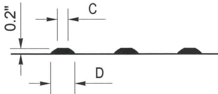
SECTION VIEW
