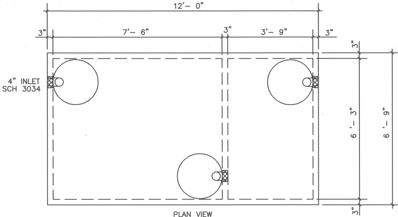
PLAN VIEW
